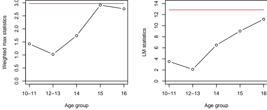
Figure 3: Fluctuation processes for the WDM_o statistic (left panel) and the \max LM_o statistic (right panel), arising from the GQ-6 data.
