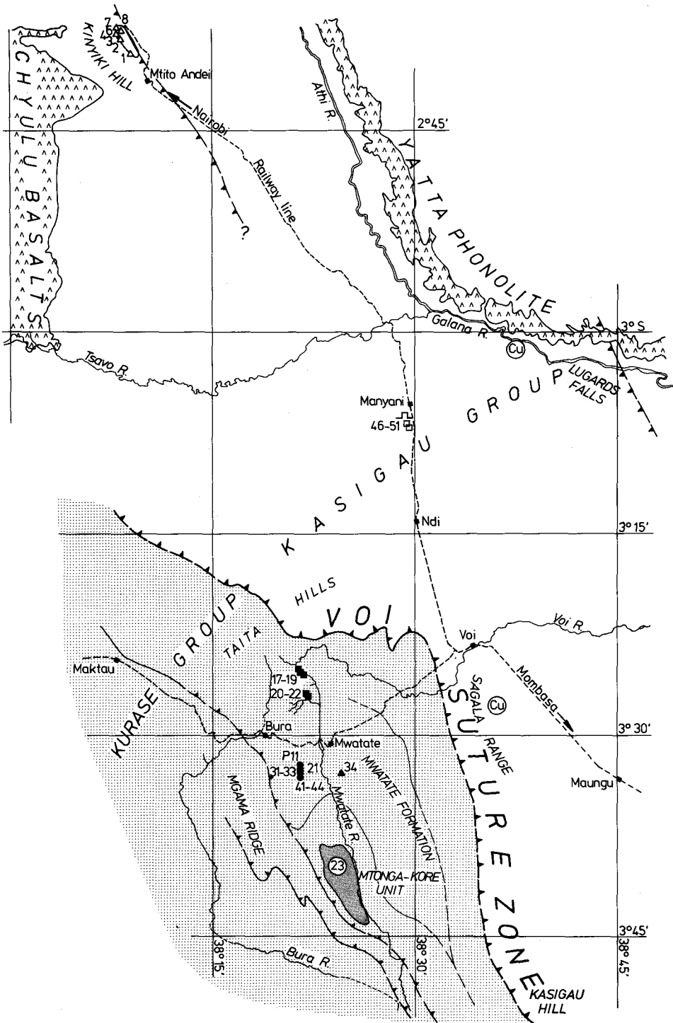
Fig. 3: Tectonic sketch map of the Mtito Andei - Taita Hills area with sample locations (thick dotted lines represent thrusts marked by ultramafic-mafic bodies; sample numbers correspond to Table 2).
